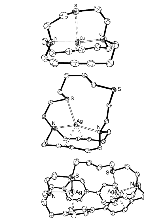
Figure 5. Molecular structures of 4 ·Cu + (top), 8 ·Ag + and 10 ·2(Ag + ) (bottom).
