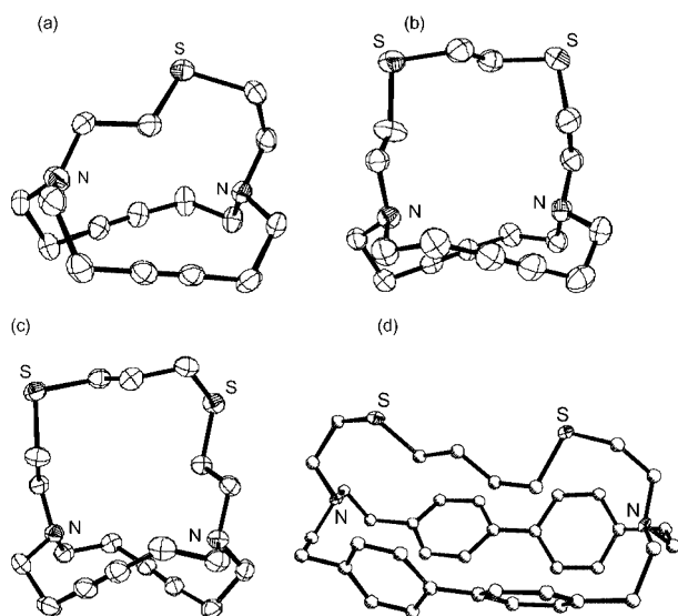
Figure 3. Molecular structures of 4 (a), 6 (b), 7 (c) and 10 (d).
