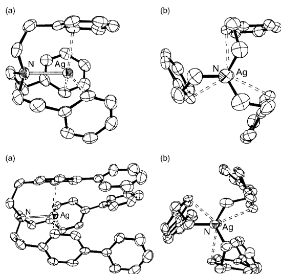
Figure 4. Molecular structures of 28 ·Ag + (top) and 33 ·Ag + in a front view (a) and a view along the N–Ag axis (b).
