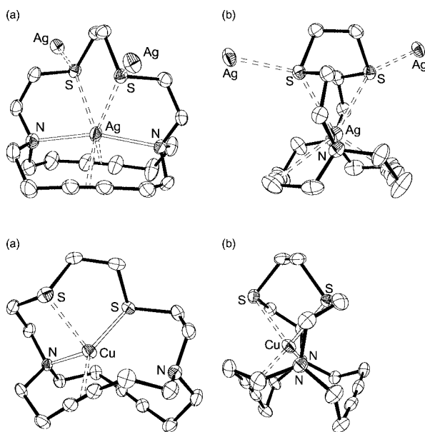
Figure 6. Molecular structure of 6\cdot\text{Ag}^+ (top) and 6\cdot\text{Cu}^+ (bottom) in a front view (a) and a view along the N–N axis (b). The hydrogen atoms are omitted for the sake of clarity.
